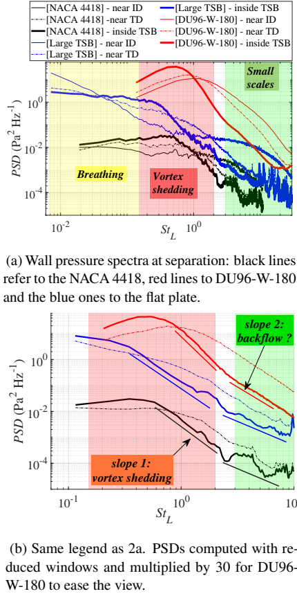
Figure 2: Power spectral densities of p_w for the three databases, upstream and downstream of separation.
