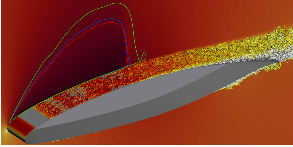
Figure 1. Isosurfaces of the swirling strength \Im(\lambda_{ci}) = 100 in the no-control case, coloured with the kinetic energy k with a white-to-red colormap in the range 0 \leq k \leq 1 . The background colour map is for the mean Mach number in the range. Lines are the sonic line M = 1 for reference (red), C1 (blue) and C2 (green).
