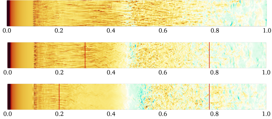
Figure 2. Instantaneous streamwise velocity component at the first grid point off the wall over the suction side, for no-control (top), C1 (middle) and C2 (bottom). The symmetric blue-to-red clourmap is for -0.1 \leq u \leq 0.1 ; the blue colour is for negative values and the red colour for positive values. The red lines mark the boundaries of the actuated region.
