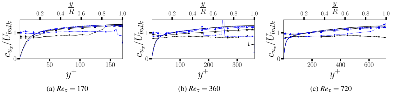
Figure 2: These figures show the approximation of mean convective velocities of the streamwise fluctuations. Black solid lines are standard pipe flow and blue dashed are drag reduced. We compare the mean velocity profile (lines with no markers), Method 1 (Method of Wills, triangles) and Method 2 (zero matching, squares).
