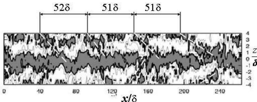
Figure 4: Figure 15 from Kitoh and Umeki, (2008) relabeled to match flow variables from the present work. Typical streak pattern on the central plane of Couette flow with Vortex Generators at Re_w = 15000 , ( Re_c = 3750 ). Dark regions \frac{|u'_{sw}|}{|U_c|} \leq -0.05 ; open regions, \frac{|u'_{sw}|}{|U_c|} \geq 0.05 .
