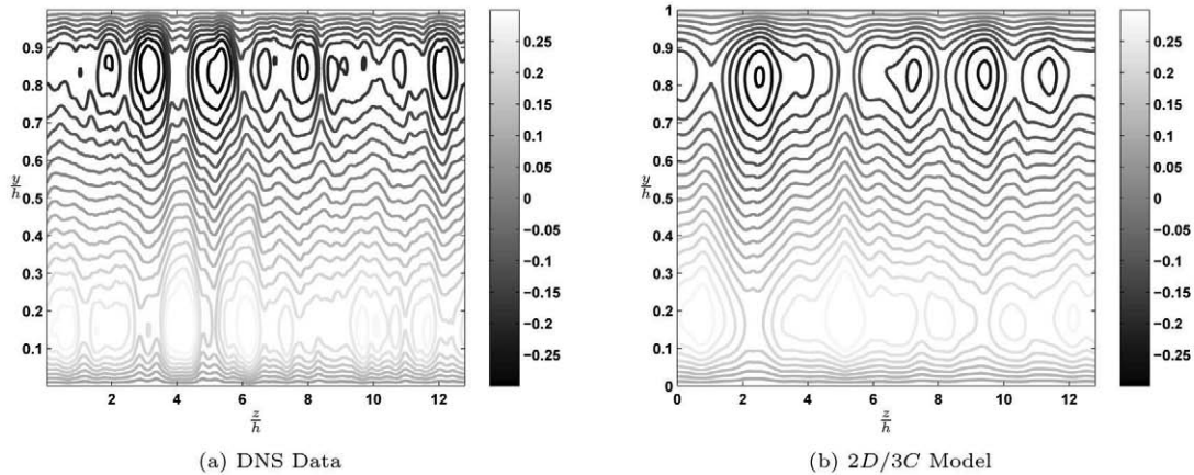
Figure 1: Contour Plots of (a) u'_{swe}(y, z) from DNS data (b) \overline{u'_{sw}(y, z, t)} from the 2D/3C model with \sigma_{noise} = 0.01 , both at Re_w = 3000 .
