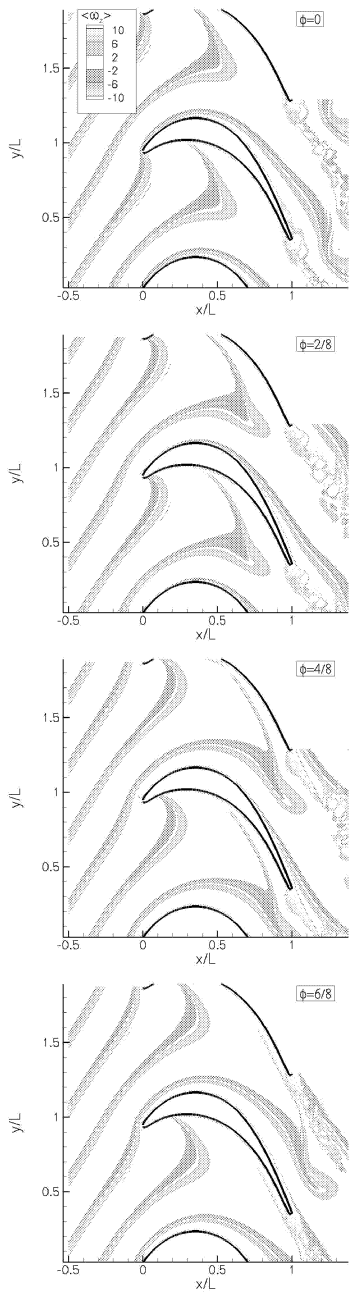
Figure 3: Contours of the phase-averaged spanwise vorticity \langle \omega_z \rangle at four different phases (Simulation B)
