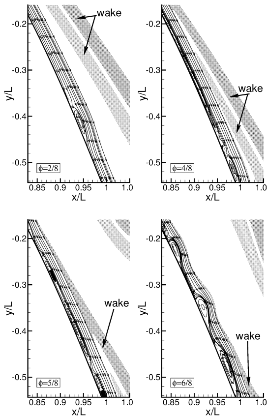
Figure 7: Simulation B: Phase-averaged snapshots showing streamlines to identify the near-wall velocity field combined with contours of the spanwise vorticity to identify the wakes.
