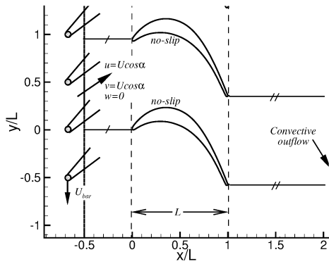
Figure 1: Cross-section at midspan of the computational domain
