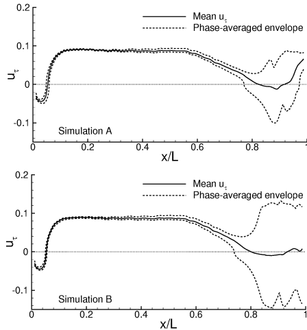
Figure 9: Mean friction velocity and its phase-averaged envelope of Simulations A and B
