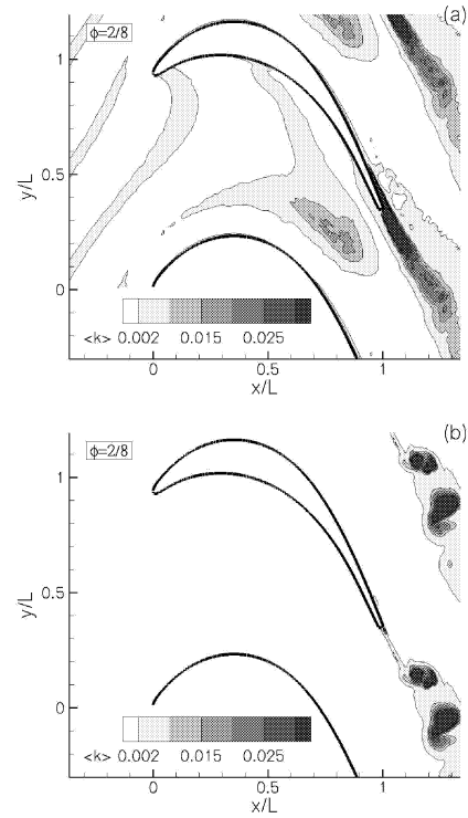
Figure 4: Contours of the phase-averaged fluctuating kinetic energy \langle k \rangle at \phi = 2/8 , (a): Simulation A, (b): Simulation B
