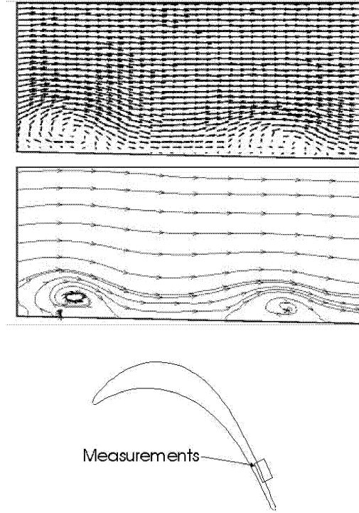
Figure 6: Experimental evidence of the Kelvin-Helmholtz instability which was found to be intermittently triggered. The upper two graphs show vector and streak lines plots of the instantaneous flow at midspan in the measurement region which is identified by the box below (from Stieger et al. 2003)
