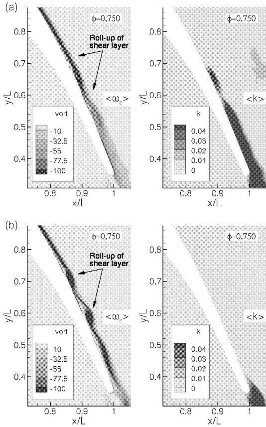
Figure 5: Contours of the phase-averaged spanwise vorticity \langle \omega_z \rangle (left) and fluctuating kinetic energy \langle k \rangle (right) both at \phi = 0.750 . (a): Simulation A, (b): Simulation B
