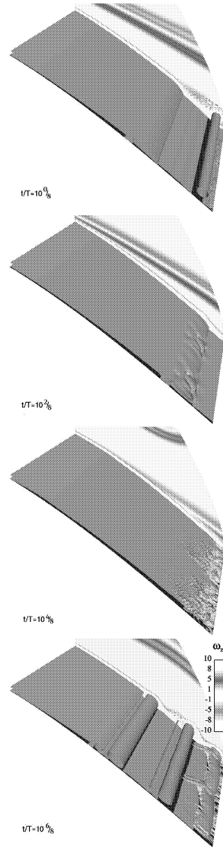
Figure 8: Simulation B: snapshots of the spanwise vorticity iso-surface \omega_z = -150 at t/T = 10\frac{0}{8}, 10\frac{2}{8}, 10\frac{4}{8} and 10\frac{6}{8} . The grey-scale contours at the back show the instantaneous spanwise vorticity and identify the wakes. Note that a disturbance-free wake consists of a positive and a negative vortex sheet adjacent to one another.
