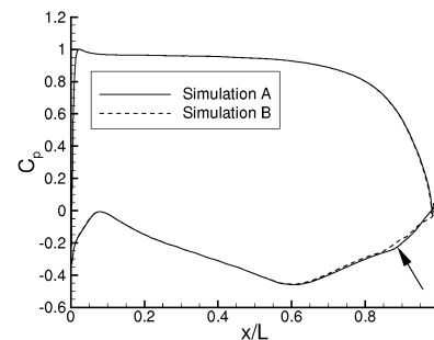
Figure 2: Mean wall static-pressure coefficient C_p = \frac{2(P - P_{ref})}{U_{ref}^2}
