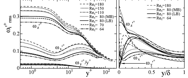
Figure 5: R.m.s. of vorticity fluctuation
