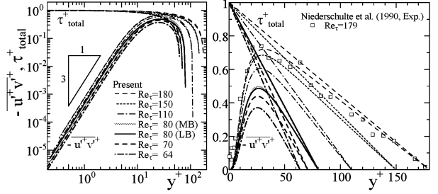
Figure 6: Reynolds shear stress and total shear distribution
