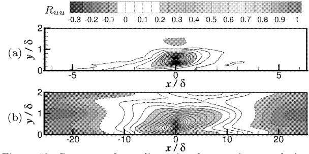
Figure 13: Contours of two-dimensional two-point correlation coefficient R_{uu} in the (x, y) -plane; the reference point is at the mid-height y_{ref} = 0.5\delta . The direction of the mean flow is from left to right. (a) Re_\tau = 180 ; (b) Re_\tau = 80 (LB). —, positive correlation; - - -, negative correlation; the line of R_{uu} = 0 is not shown here. Contour interval \Delta R_{uu}:0.05 .
