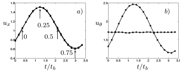
Figure 2: Phase-averaged velocity at the inflow plane x/R = -2 at r/R = 0.75 , i.e. in the middle of the annular duct, as a function of time over one period. a) Axial component \tilde{u}_x/U_b and phases discussed below. b) Tangential component \tilde{u}_\theta/U_b . Sim.2: circles. Sim.3: squares.
