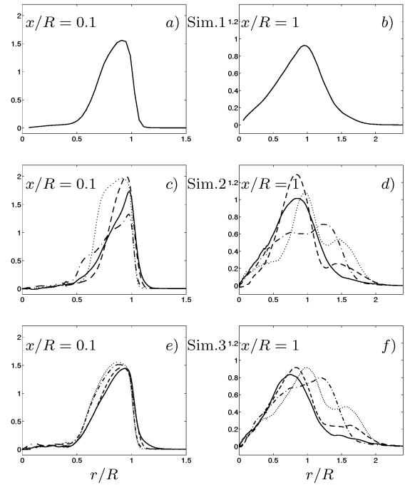
Figure 4: Profiles of tangential velocity u_\theta/U_b at x/R = 0.1 (left) and x/R = 1 (right). a – b ) Time-averaged velocity in Sim.1. c – d ) Phase-averaged velocity in Sim.2. e – f ) Phase-averaged velocity in Sim.3. Phases as indicated in Fig.2. Key to lines is given in Table 2.
