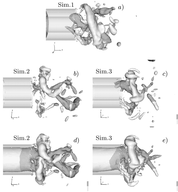
Figure 8: Instantaneous coherent structures at \psi = 0.25 (arbitrary phase with Sim.1). a – c ) Iso-surface p'' = -0.3 , d – e ) Iso-surface p = -0.5 for the same data sets. The color is determined by the sign of the radial gradient of the phase-averaged axial velocity (in Sim.1 the time-average).
