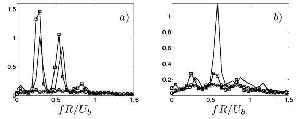
Figure 9: PSD of velocity fluctuations. a ) PSD of axial velocity fluctuations at x/R = 0.1 , r/R = 0.6 . b ) PSD of radial velocity fluctuations at x/R = 0.9 , r/R = 1.2 . Solid line: Sim.1, circles: Sim.2, squares: Sim.3. Arbitrary units are used in the vertical axis.
