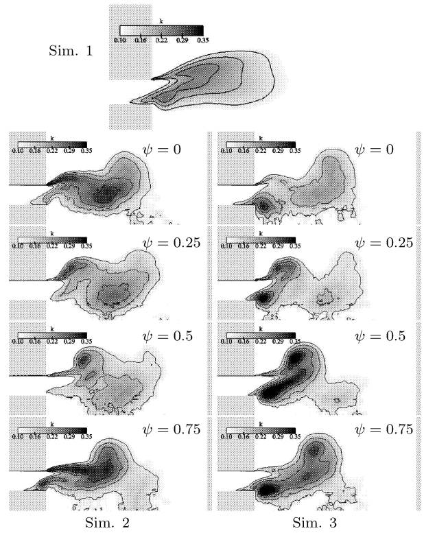
Figure 7: Turbulent kinetic energy k/U_b^2 contour plots in a plane \theta = \text{const} . Top 1: Sim.1. Left: Sim.2, Right: Sim.3.
