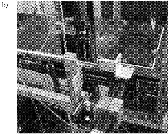
Figure 2 Experimental setup. a) Turbulent air channel flow facility and DSP control system, b) Test section and LDV traversing mechanism.
