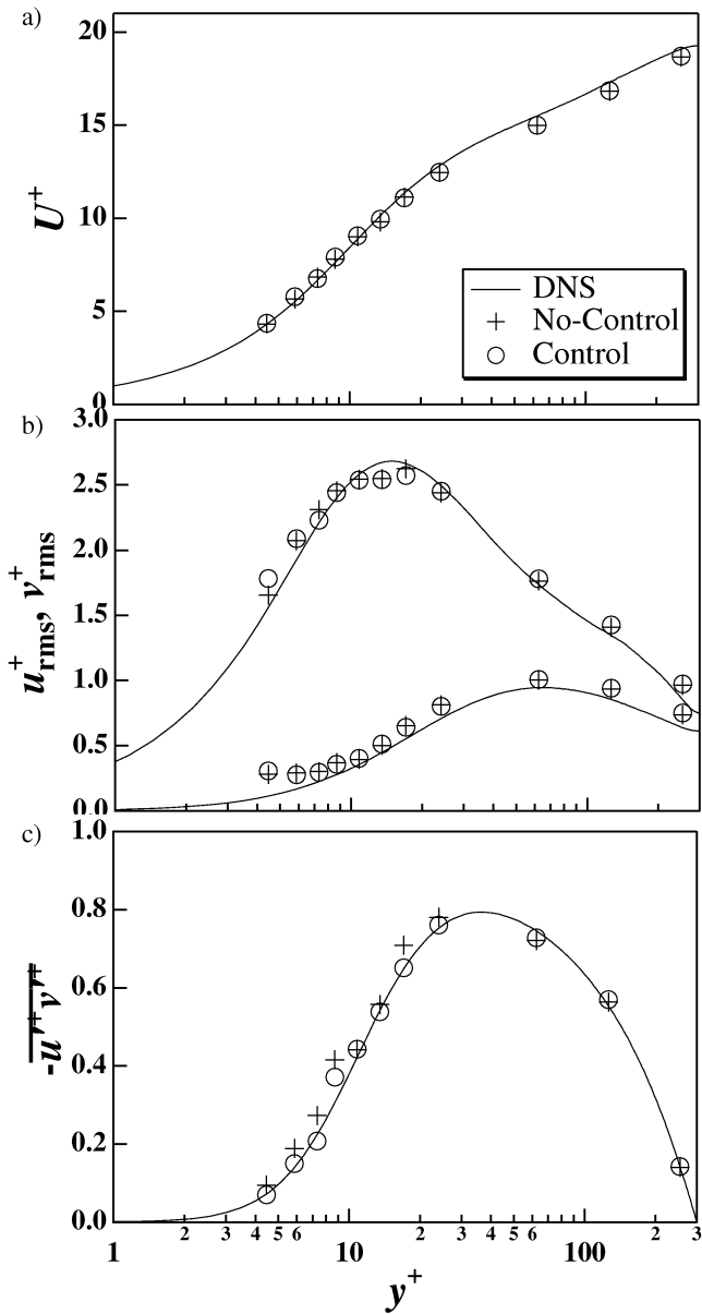
Figure 5 Turbulent statistics above the center of an actuator measured with LDV. a) Mean velocity profile, b) RMS values of turbulent fluctuations, c) Reynolds shear stress. The wall friction velocity is estimated for unmanipulated flow.
