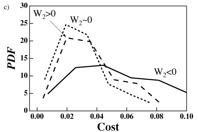
Figure 4 Result of GA-based feedback control in a turbulent channel flow. a) Cost function versus generation, b) Optimum weight, c) Probability density of J depending on the sign of W_2 .
