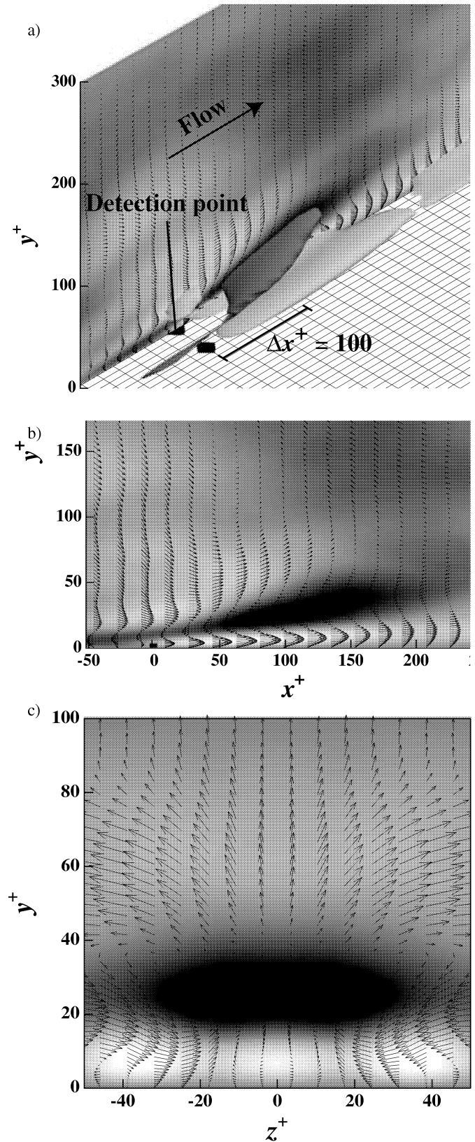
Figure 7 Conditional-averaged velocity field associated with events q > q_{rms} . a) Bird's eye view, b) Contours in the x - y plane, c) Contours and the cross-stream vectors in the y - z plane at x^+=100 . Black to white, \langle u^+ \rangle = -0.5 to 0.5 . DNS database of an unmanipulated channel flow at Re_\tau=300 is employed in order to extract the flow structures.
