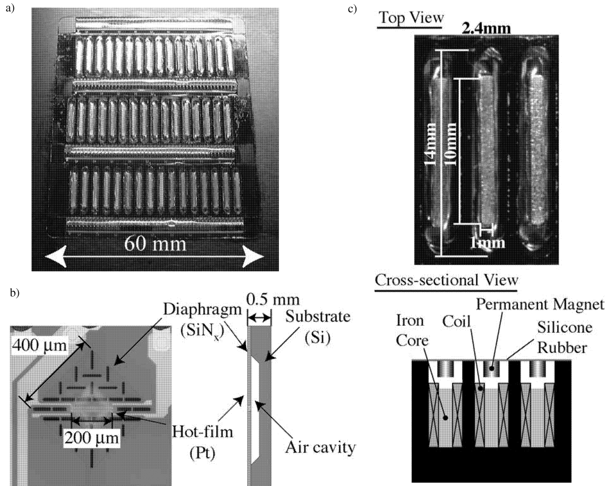
Figure 1 Prototype feedback control system for wall turbulence. a) Plane view of the system having 192 wall shear stress sensors and 48 wall-deformation actuators, b) Magnified view of a sensor, c) Magnified view of actuators.
