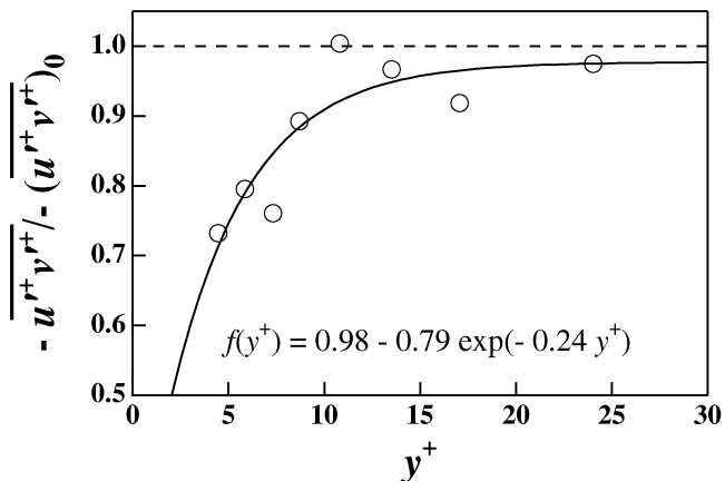
Figure 6 Normalized Reynolds stress profile close to the wall.
