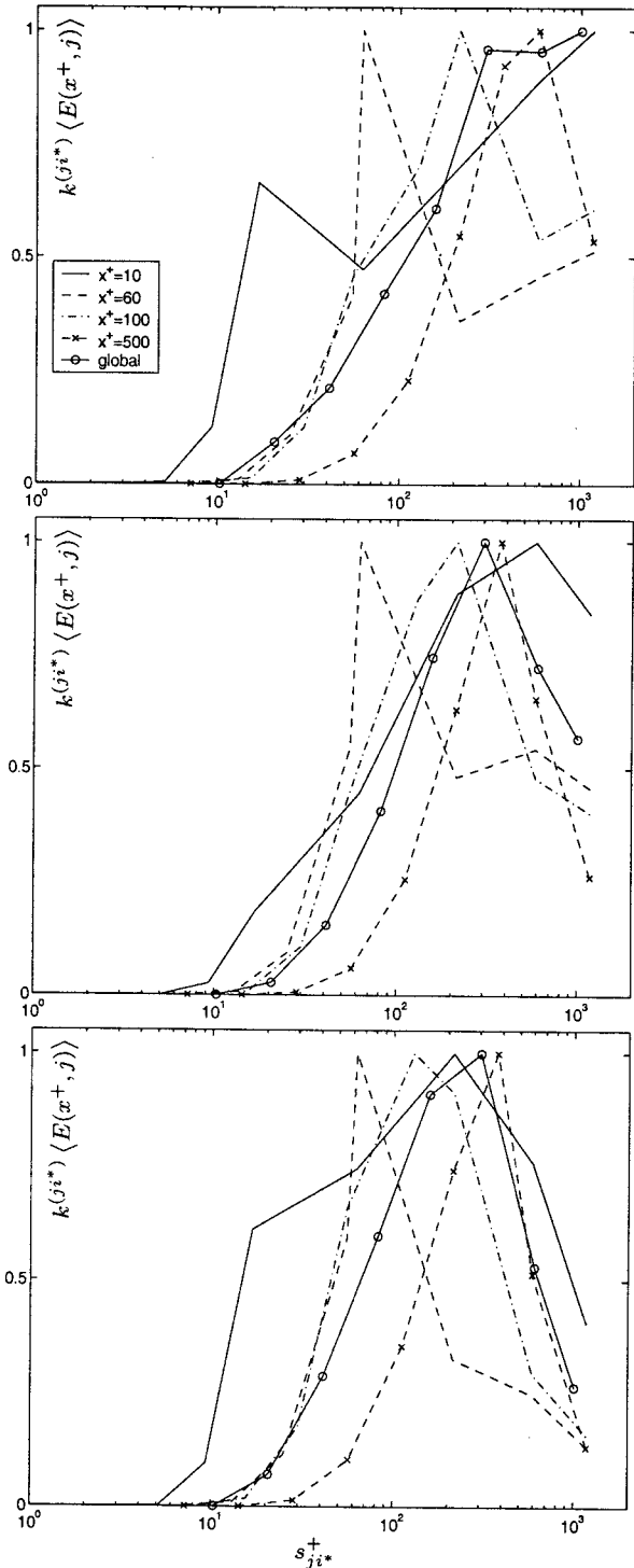
Figure 5: Global and local pre-multiplied power spectra obtained from statistics of the transform of velocity fluctuations recorded along the wall-normal direction in plane channel flow at Re_\tau = 590 . Top: streamwise velocity component; center: wall-normal component; bottom: spanwise component. All curves are normalized by their maximum value.
