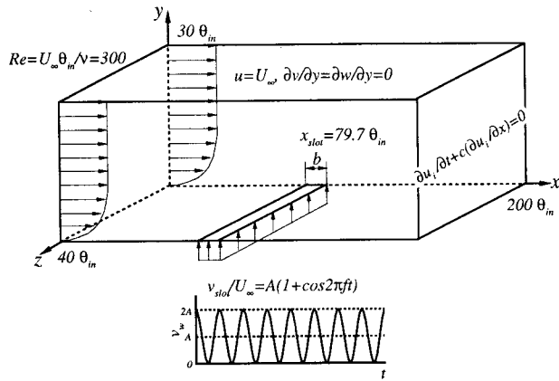
Figure 1: Schematic diagram of the computational domain.
