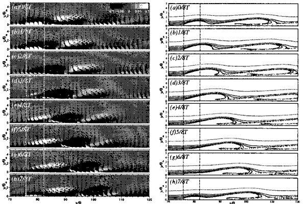
Figure 5: Contour plots of the oscillating components of spanwise vorticity with the oscillating components of velocity vectors (left) and streaklines (right) for A^+=0.5 .
