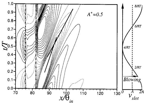
Figure 4: Spatio-temporal evolution of the relative modulations of wall shear stress ( A^+=0.5 ). The contour levels range from -1 to 1 by increments of 0.1.
