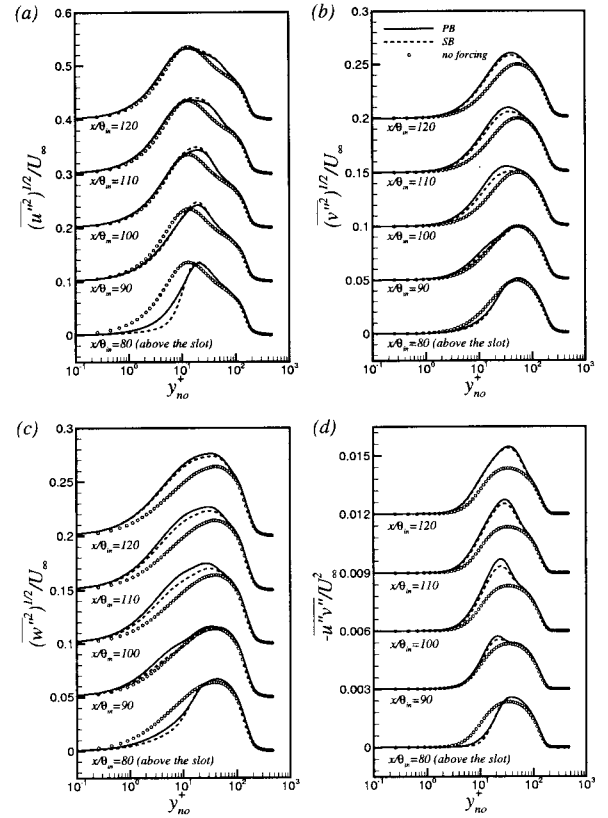
Figure 7: Variations of time-averaged turbulent intensities and Reynolds shear stress for A^+ = 0.5 . (a) u''_{rms} , (b) v''_{rms} , (c) w''_{rms} , (d) -\overline{u''v''} .
