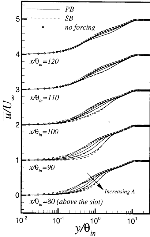
Figure 3: Time-mean velocity profiles.
