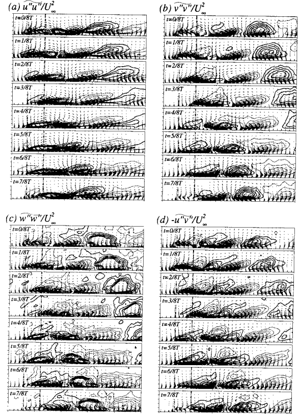
Figure 9: Contours of the oscillating component of turbulent intensities and Reynolds shear stress ( A^+ = 0.5 ). Contour levels are from -0.004 to 0.004 by increments of 0.0008 for \overline{u''^2}/U_\infty^2 , and from -0.001 to 0.001 by increments of 0.0002 for \overline{v''^2}/U_\infty^2 , \overline{w''^2}/U_\infty^2 and -\overline{u''v''}/U_\infty^2 . The plot domain is 70 \leq x/\theta_{in} \leq 120 and 0 \leq y/\theta_{in} \leq 5 .
