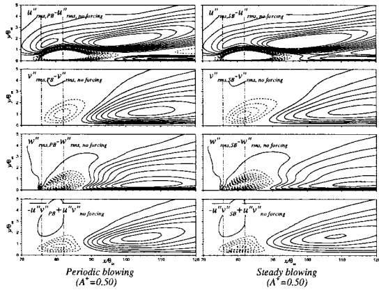
Figure 6: Contours of the differences of the time-averaged rms velocity fluctuations and Reynolds shear stress. Contour levels are from -0.02U_\infty to 0.02U_\infty by increments of 0.002 for the velocity fluctuations, and from -0.002U_\infty^2 to 0.002U_\infty^2 by increments of 0.0002 for the Reynolds shear stress.
