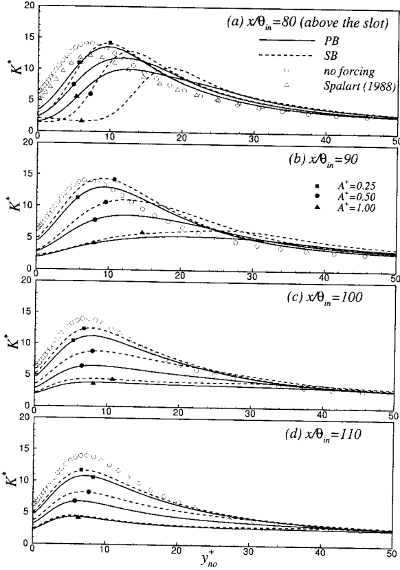
Figure 8: Variations of the energy partition parameter K^* = 2\overline{u''^2} / (\overline{v''^2} + \overline{w''^2}) .
