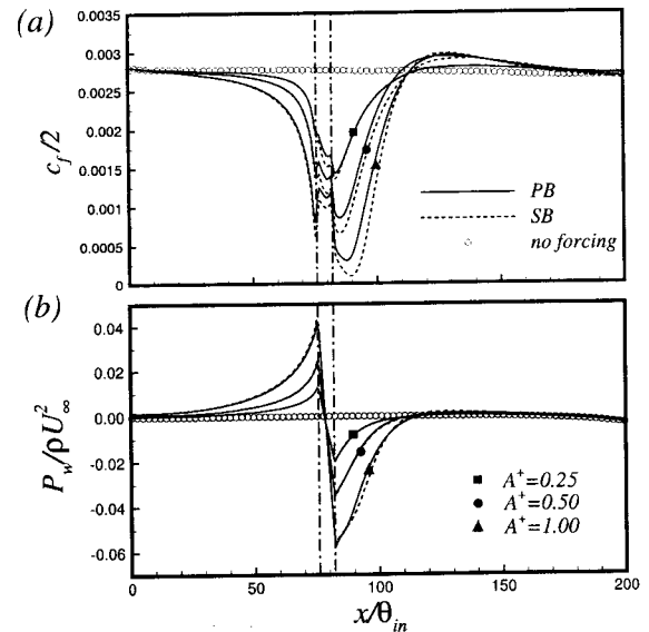
Figure 2: Variations of c_f and P_w for three forcing amplitudes.
