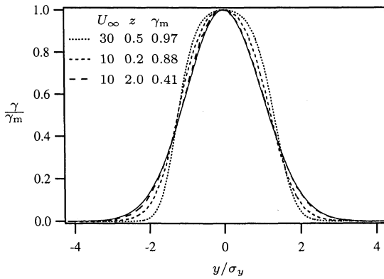
Figure 7: Normalized lateral profiles of concentration intermittency for C_T = 0.002C_0 . Units in the legend are in terms of cm.
