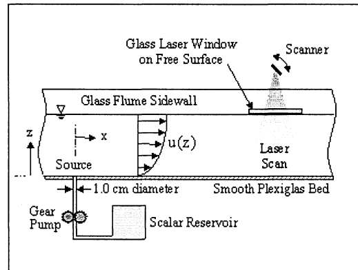
Figure 2: Side view of the flume test section showing the scalar source configuration and the imaging apparatus.
