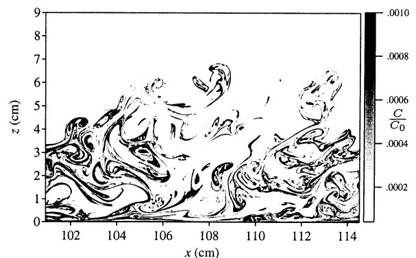
Figure 1: Image of the instantaneous normalized concentration structure in a thin vertical slice through the centerline of a scalar plume developing in a turbulent boundary layer. The scalar source is at x = 0 , z = 0 . Flow is from left to right.
