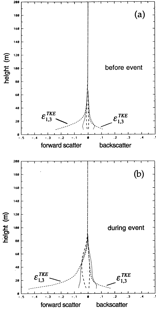
Figure 5. Vertical profiles of TKE transfer by component (1,2: dotted line; 1,3: short dashed line; 2,3: long-dashed line) for periods (a) before and (b) during enhanced turbulence; units are 0.01 \text{ m}^2/\text{s}^3 .
