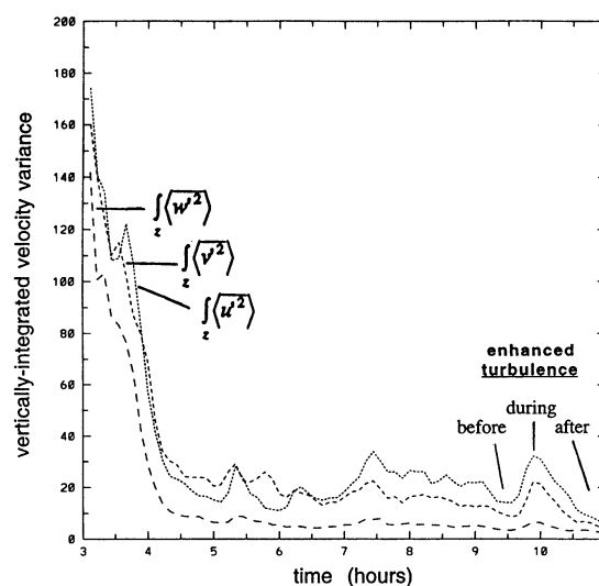
Figure 4. Time series of vertically-integrated velocity variance by component.
