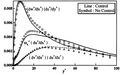
Figure 12. Production term in the streamwise vorticity equation.
