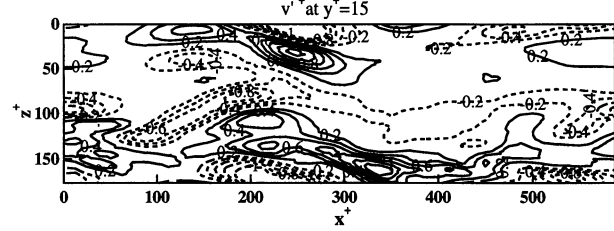
Figure 13. Instantaneous wall-normal velocity at y^+ = 15 .
