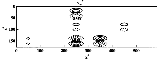
Figure 14. Instantaneous wall velocity.
