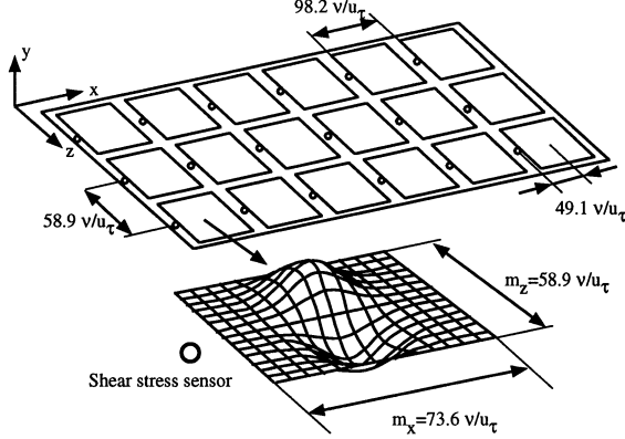
Figure 10. Arrangement of deformable actuators.
