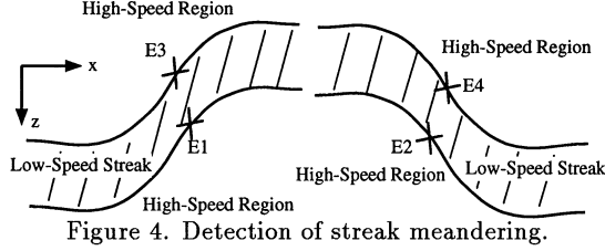
Figure 4. Detection of streak meandering.
