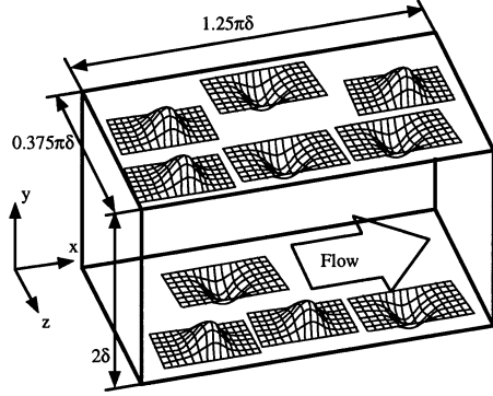
Figure 1. Flow geometry and coordinate system.
