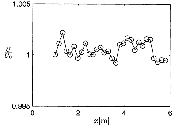
Figure 2: Streamwise mean velocity distribution outside of the boundary layer.
