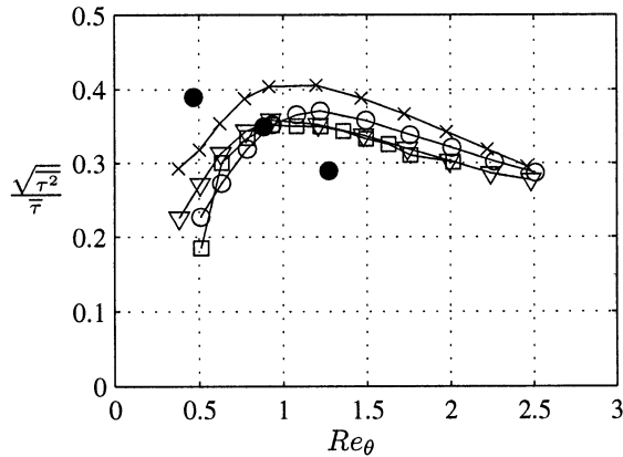
Figure 11: Fluctuating wall shear-stress intensity. \circ : wall-wire l = 500 \mu m , \square : wall-wire l = 200 \mu m , \triangle : MEMS hot-film l = 150 \mu m , \times : wall-wire l = 250 \mu m , \bullet : wall-wire l = 750 \mu m (Alfredsson et al., 1987).
